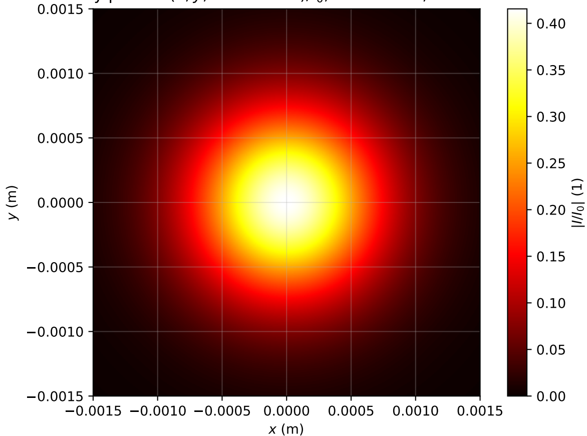
Intensity profile I(x, y, z = 3.821m)/I_0 , P_{in}=0.5P_{cr} , artificial time
